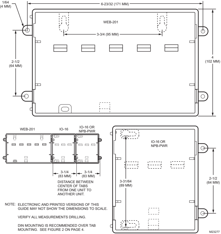
Fig. 1. Tab mounting dimensions in inches (mm).
