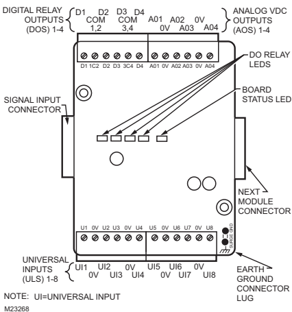
Fig. 3. WEB-IO-16 Wiring terminal locations.
