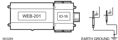
Fig. 4. WEB-IO-16 earth ground connection.
