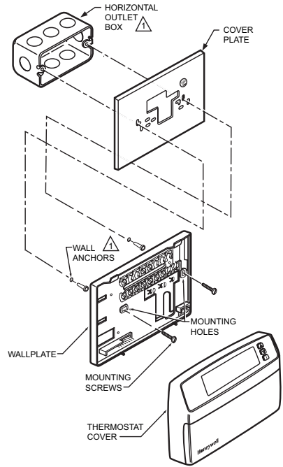
Fig. 2. Mounting cover plate and thermostat wallplate on horizontal outlet box or directly on wall.
