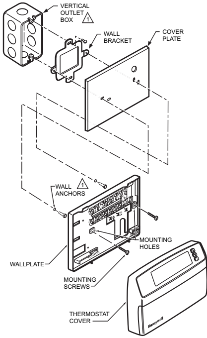
Fig. 1. Mounting wall bracket, cover plate and thermostat wallplate on vertical outlet box.
