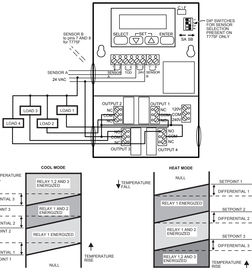
Fig. 28—Four-stage control, 24 Vac input; 24 Vac load.
