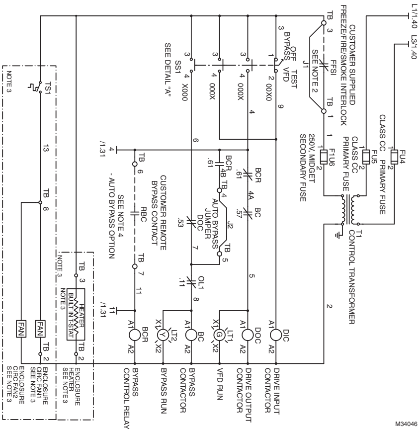
Fig. 4. Frame 8, 3 Contactor Auto-bypass Wiring Diagram.
