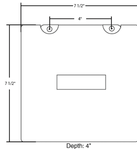
Fig. 1. Enclosure dimensions (front view).
